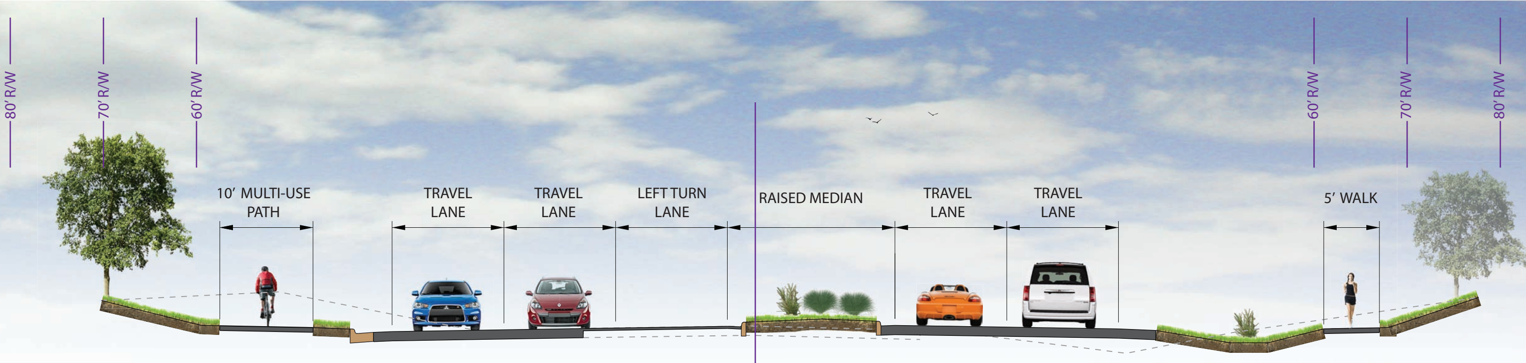
Raised Median Section South Old State Road - County Road 10
