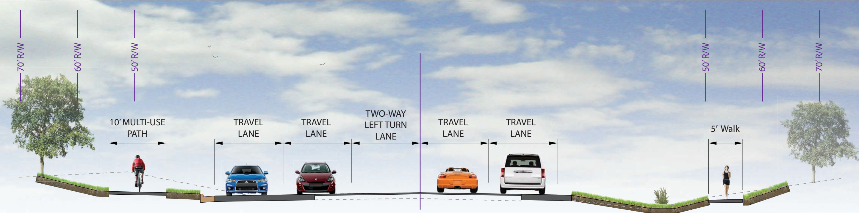
5 Lane Section South Old State Road - County Road 10
